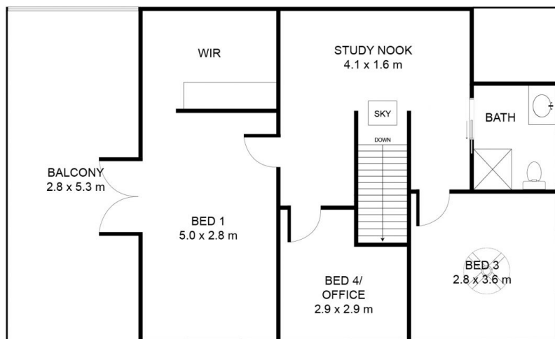
FIRST LEVEL
